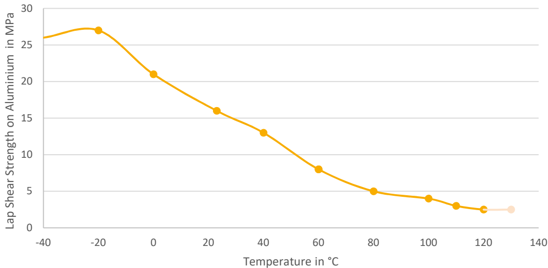
Lap Shear Strength on Aluminium versus Temperature
